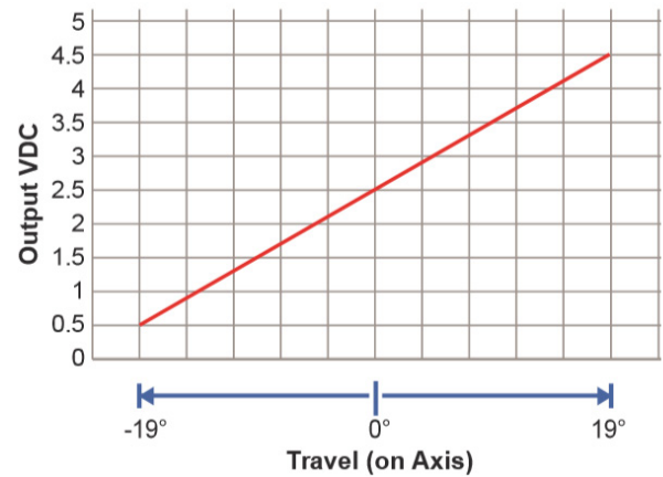
Micro Joystick Travel Output VDC
