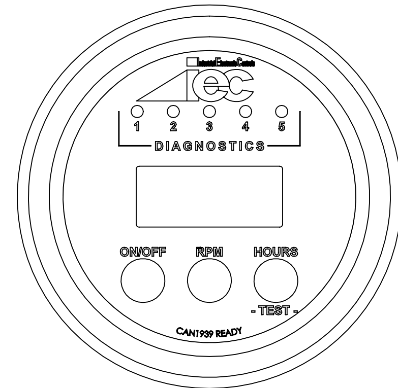
VIEW A-A SCALE 1 : 1
